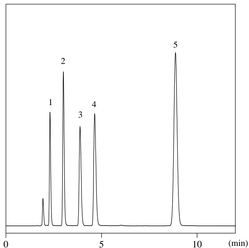
Fig. Chromatogram of ingredients in cold medication
