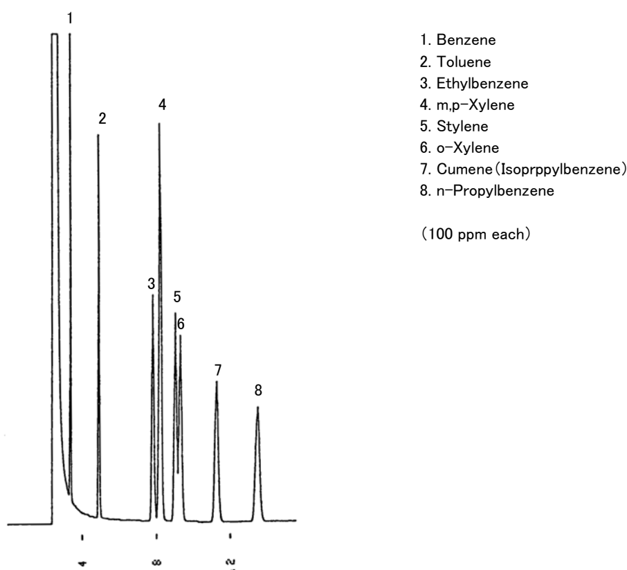
Fig. Chromatogram of Aromatic hydrocarbons.
