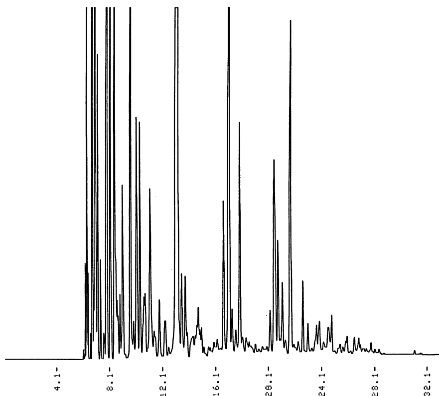
Fig. Chromatogram of Gasoline.
