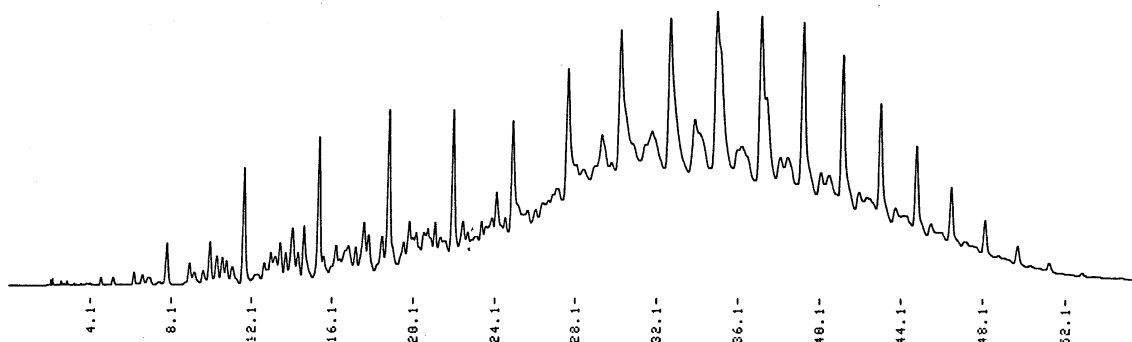
Fig. Chromatogram of Light oil.
