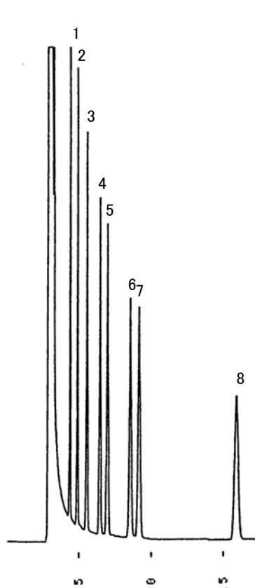
Fig. Chromatogram of Ketones.
