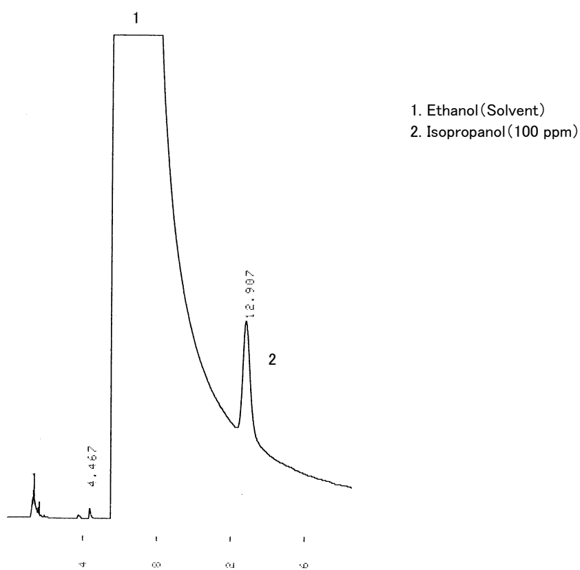
Fig. Chromatogram of Trace constitutes in organic solvent.
