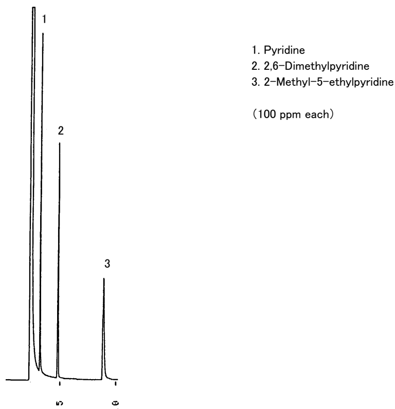
Fig. Chromatogram of Pyridines.
