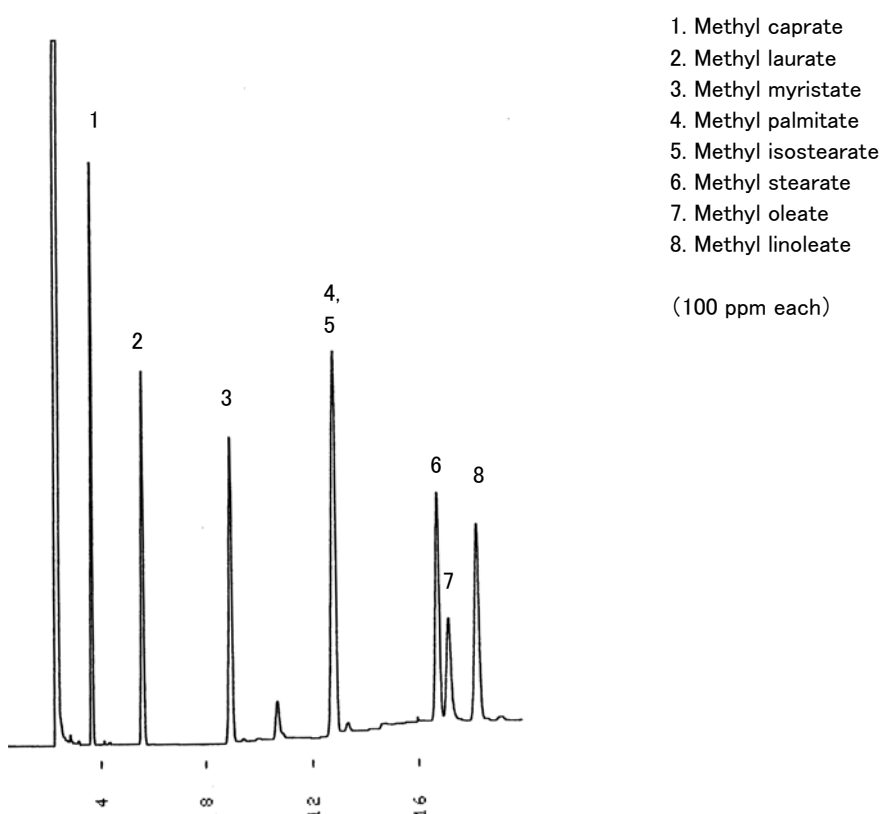
Fig. Chromatogram of Fatty acids.
