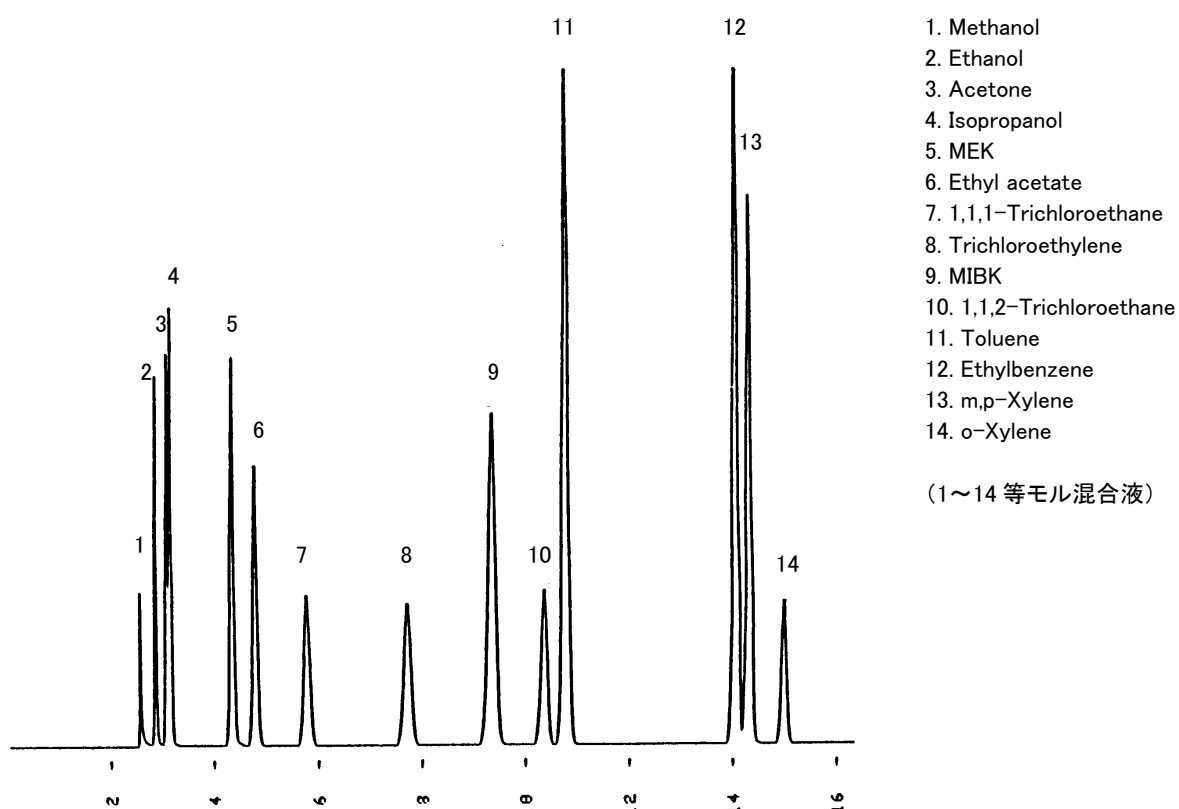
Fig. Chromatogram of Organic solvents in working environment assessment.
