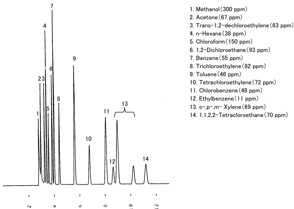
Fig. Chromatogram of Organic solvents in working environment assessment.
