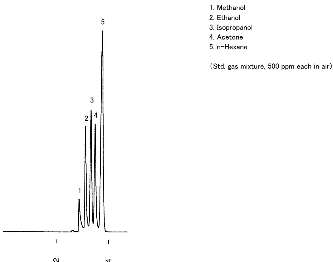
Fig. Chromatogram of Organic solvents.
