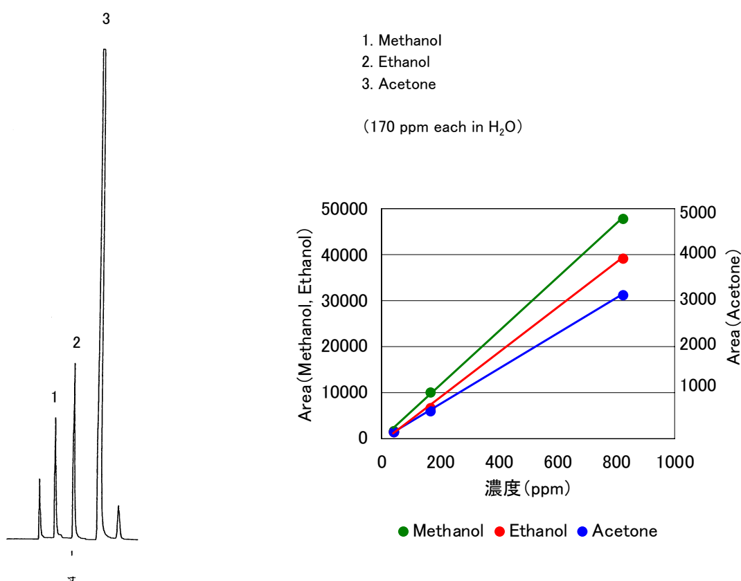
Fig. Chromatogram of Organic solvents in water.
