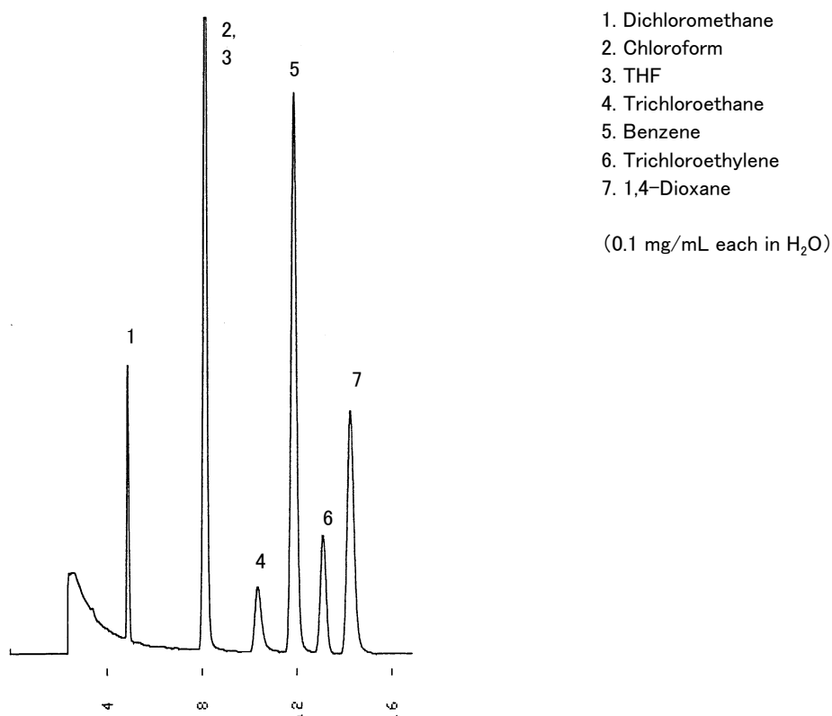
Fig. Chromatogram of Organic solvents in water.
