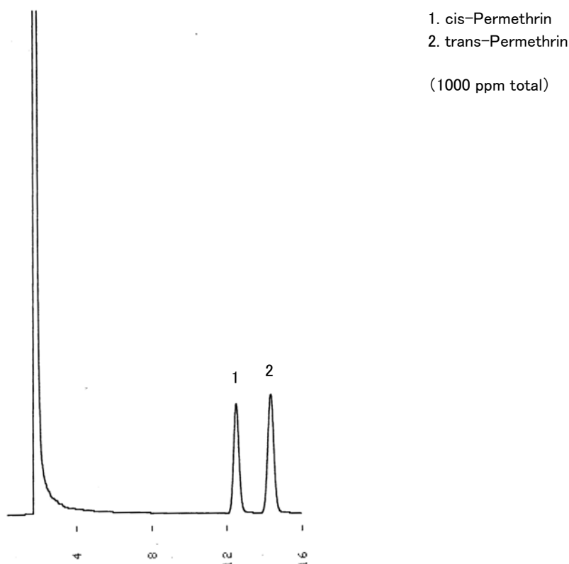
Fig. Chromatogram of Stereoisomer.
