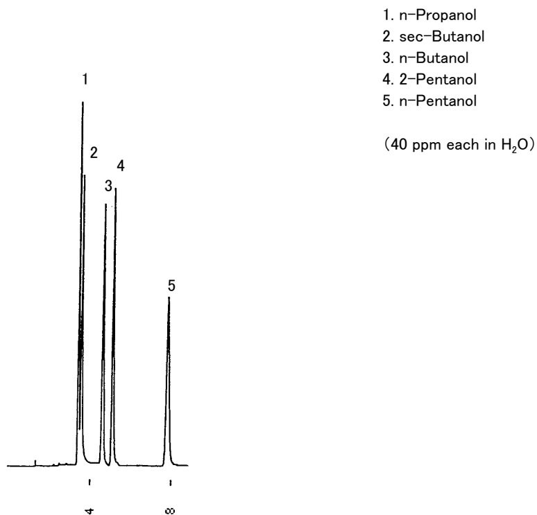
Fig. Chromatogram of lower alcohols in water.
