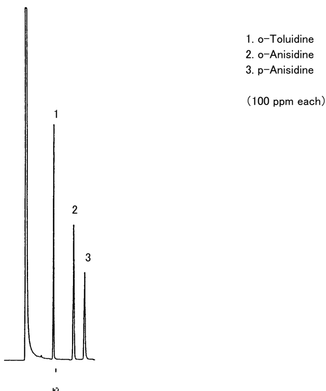
Fig. Chromatogram of Anisidines.
