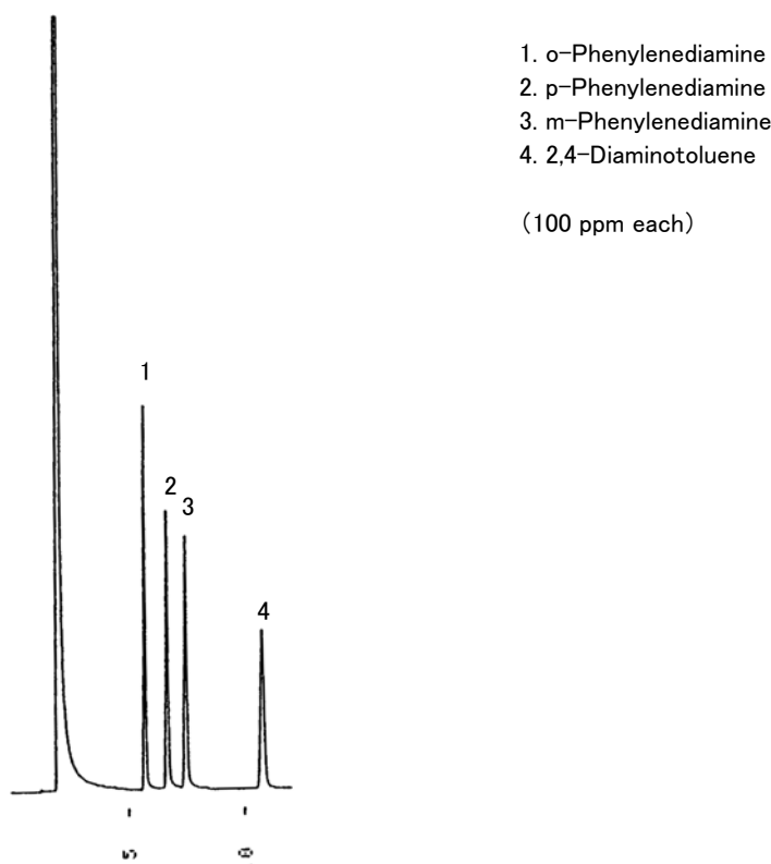
Fig. Chromatogram of Aromatic diamine.
