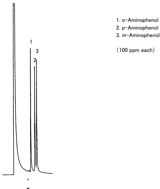
Fig. Chromatogram of Aminophenol.
