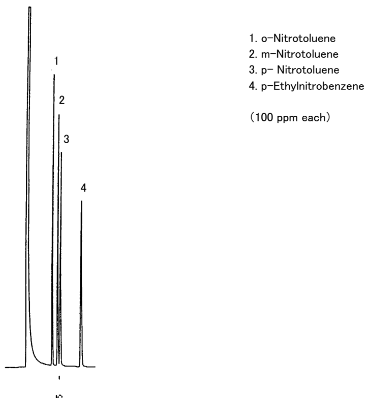
Fig. Chromatogram of Aromatic nitro compounds.
