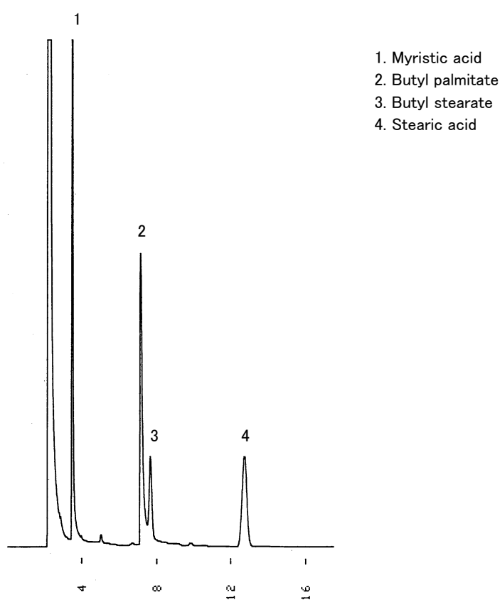
Fig. Chromatogram of Fatty acids.
